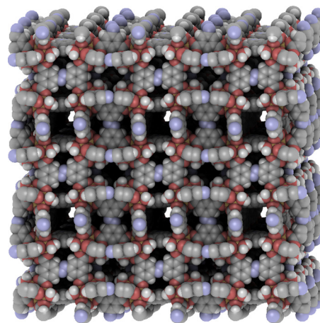
Fig. 5 PCN-250' or Fe 2 -AzBTC (CSD code TOWPEC). Created with iRASP. 39
